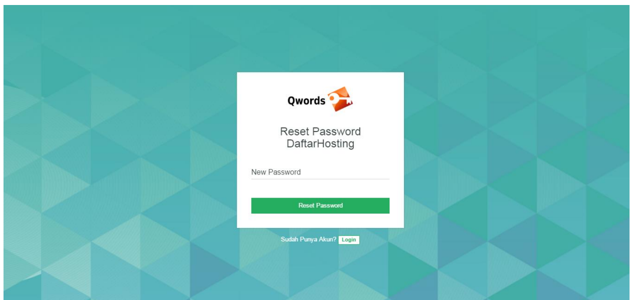
Gambar 4.4 Lupa Password
