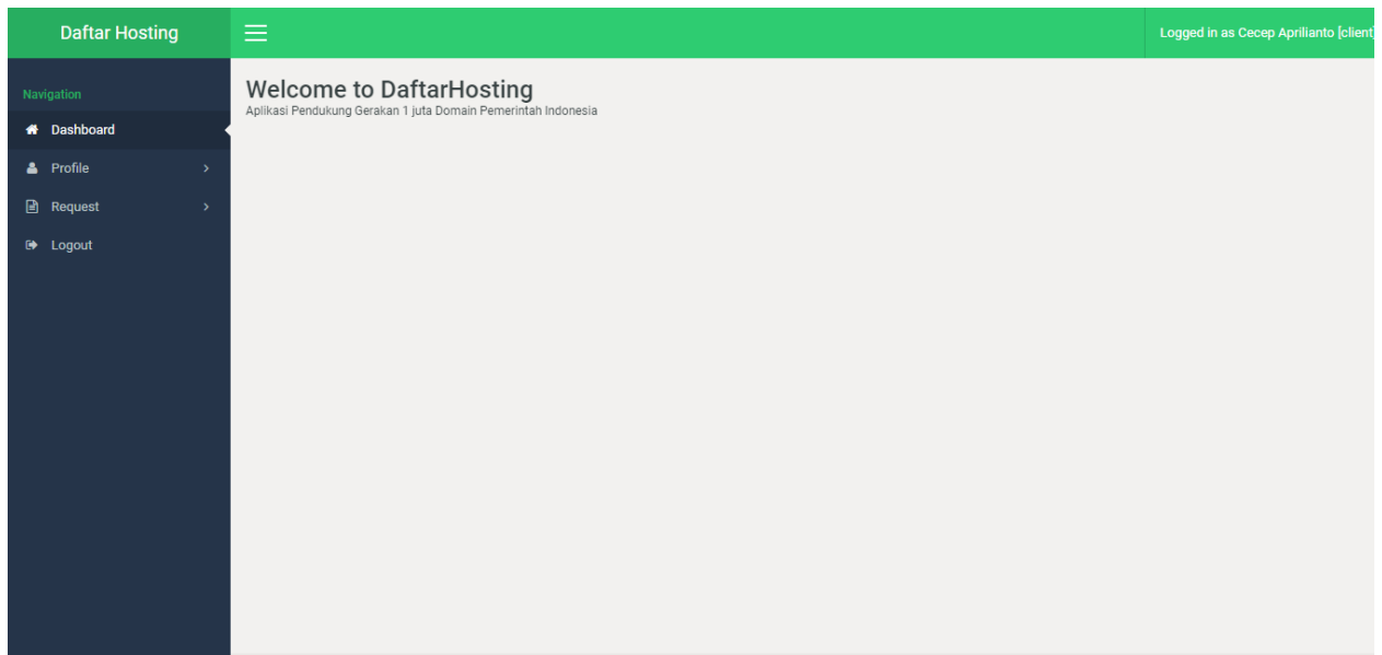
Gambar 5.1 Dashboard
