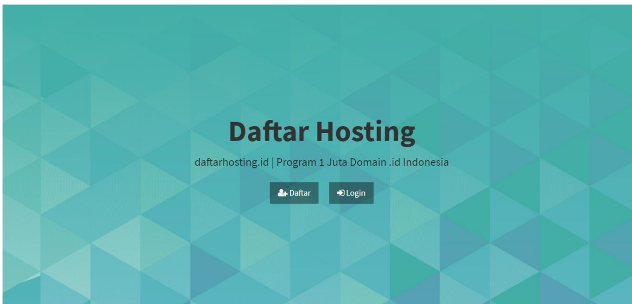
Gambar 1.1 Home
